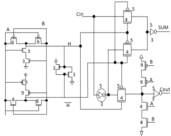
Figure 3: Proposed Full adder
