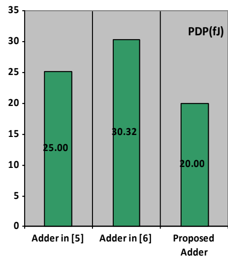
Figure 6: PDP results in 4 bit RCA for V_{dd}=1.1\text{V} , C_L=2\text{ fF} and Frequency = 50MHz
